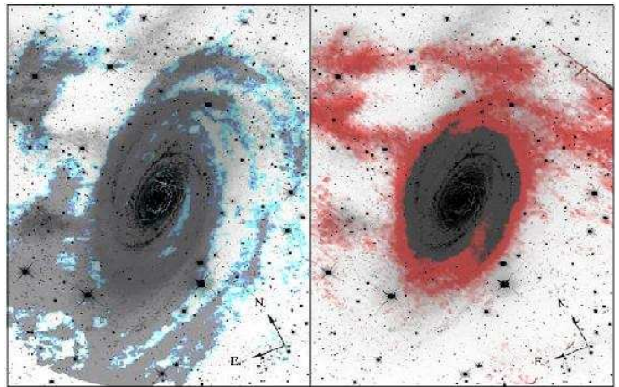
Fig. 5. HOA images of the region around M81. The HI emission from Walter et al. (2008) (left panel) and the MIPS 160\mu\text{m} image (right panel) have been overplotted.
