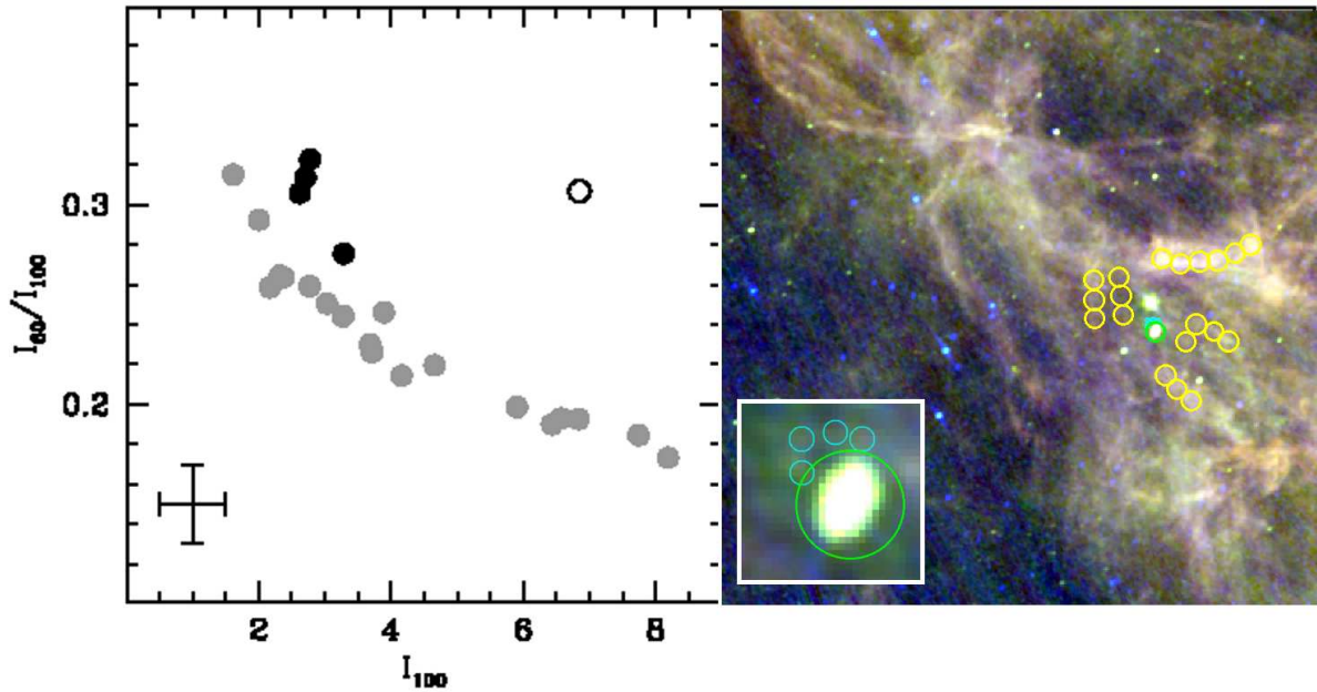
Fig. 3. In the left panel the I_{60\mu m}/I_{100\mu m} ratio is shown as a function of the I_{100\mu m} brightness for the loop (black filled points), M81 (open point) and the surrounding cirrus features (grey points). The typical uncertainty of the regions along Arp’s loop is shown in the bottom part of the panel. The right panel depicts a false-color IRAS image of the M81 region. North is up, east is to the left. The circular apertures used in the analysis of the Galactic cirrus (yellow circles; 12’ diameter), M81 (green circle; 12’ diameter) and Arp’s loop (tiny cyan circles above M81; 4’ diameter) are shown. A zoom into the M81 region is shown in the inner box.
