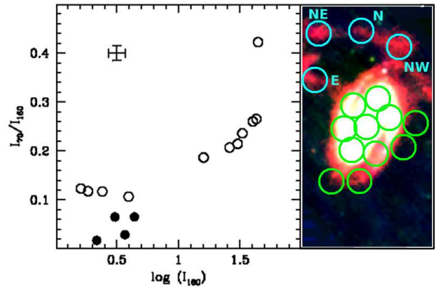
Fig. 4. In the left panel the I_{70\mu m}/I_{160\mu m} ratio calculated for Arp’s loop (filled circles) and the M81 disk (open circles) are shown as a function of the I_{160\mu m} brightness. The typical uncertainty is shown in the upper part of the panel. In the right panel the 27'\times 41' color map of the Spitzer MIPS emission for M81 was constructed using the 24\mu m , 70\mu m and 160\mu m images. The circular apertures are also shown with the same color code used in Figure 3.
